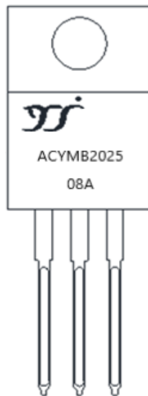
(TO-220AB-1 Package)
