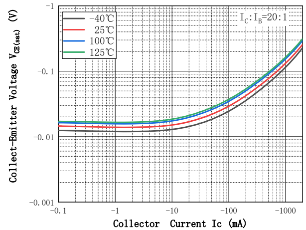
Fig.4 - Collect-Emitter Saturation Voltage
