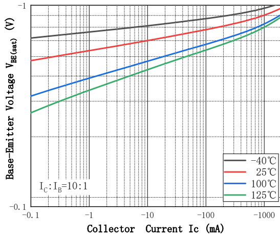
Fig.5 - Base-Emitter Voltage
