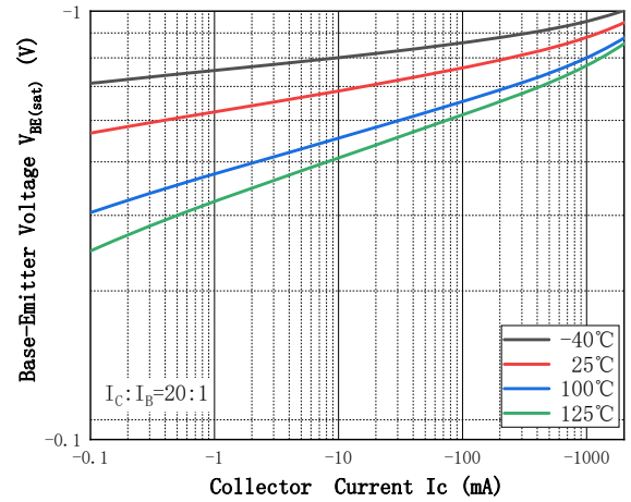
Fig.6 - Base-Emitter Voltage
