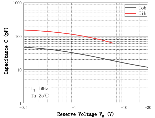
Fig.8 - Cob/Cib—VCB/VEB
