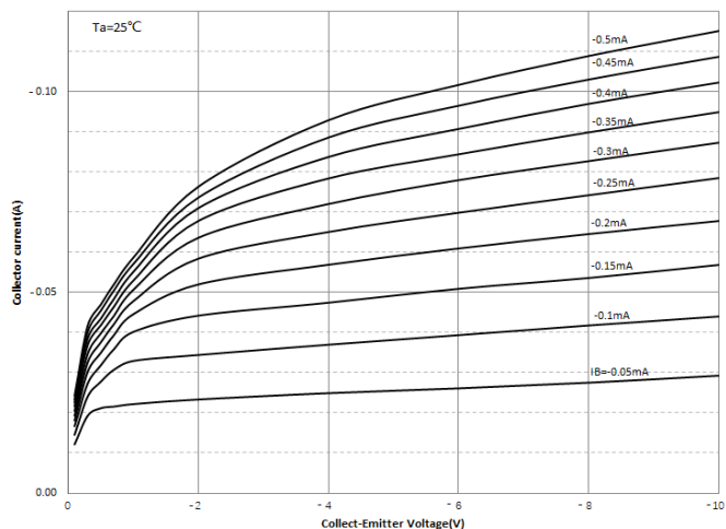
Static Characteristics
